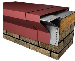
Cornice Version
