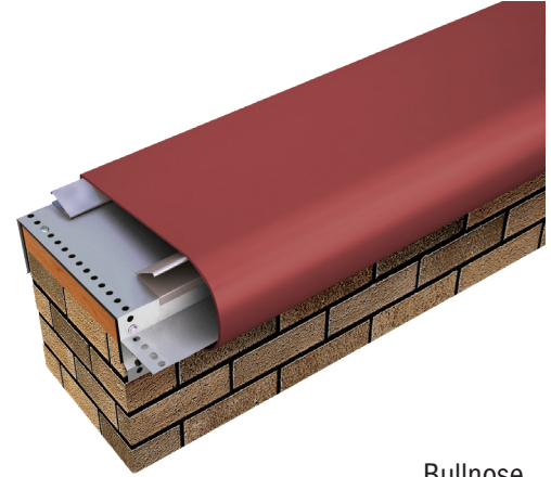
Bullnose Version
